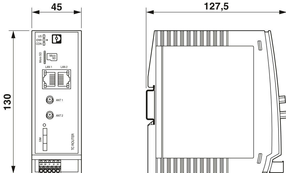
Dimensional drawing
