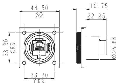
○ Cat 5e mates with PX0836, PX0837, PX0838 & PX0834 flex connectors ○ Cat 6a mates with PX0896, PX0897, PX0898 & PX0894 flex connectors ○ Standard RJ45 patchcord can be plugged into rear ○ Version with earth wire available ○ Flange fixing ○ Complete with panel sealing gasket
