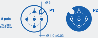
5 PINS A-CODED
