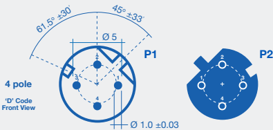
4 PINS D-CODED
