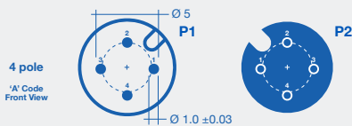
4 PINS A-CODED
