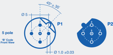
5 PINS B-CODED
